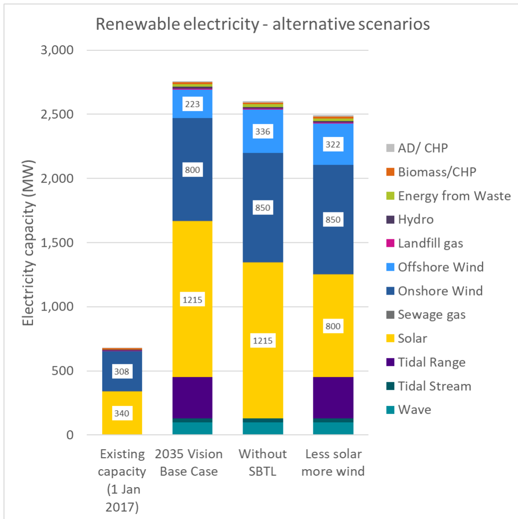
Figure 22: Alternative scenarios without tidal lagoon and with less solar
