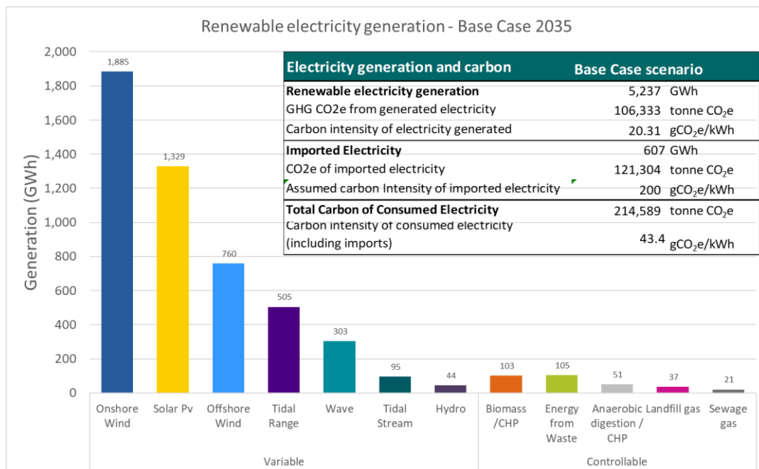
Figure 21: Energy generation by renewable technology type
