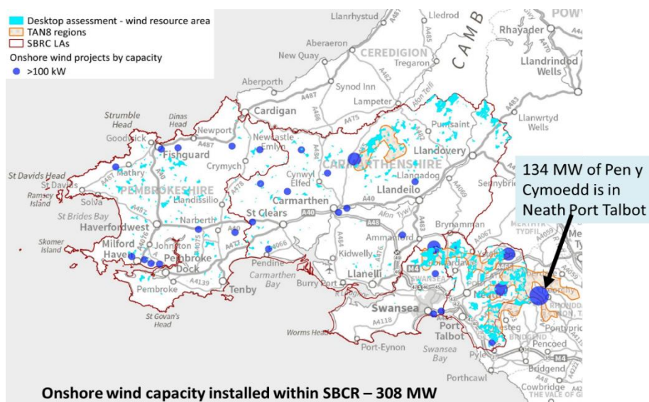
Figure 23: Wind resource areas, existing onshore wind projects and the TAN 8 SSAs in SBCR
