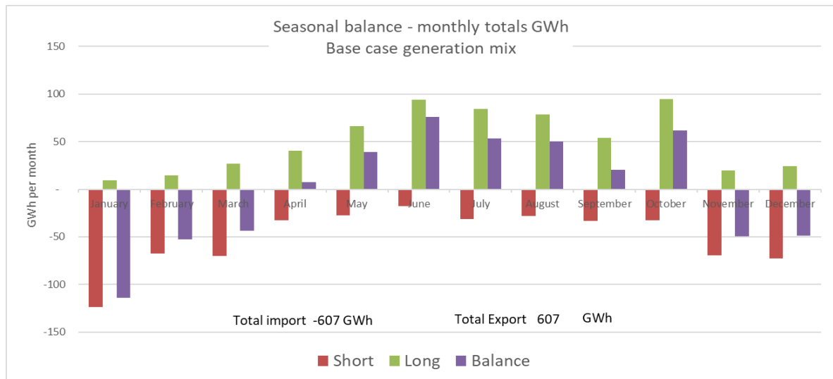
Figure 52: Monthly analysis of import and export balances
