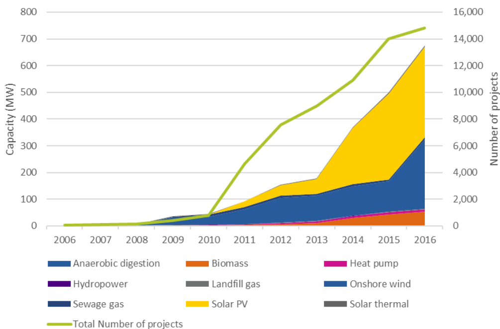
Figure 19: Renewable energy capacity and project numbers in SBCR in 2016. Data source: Welsh Government, ‘Energy Generation in Wales report’ (1 Jan 2017)
