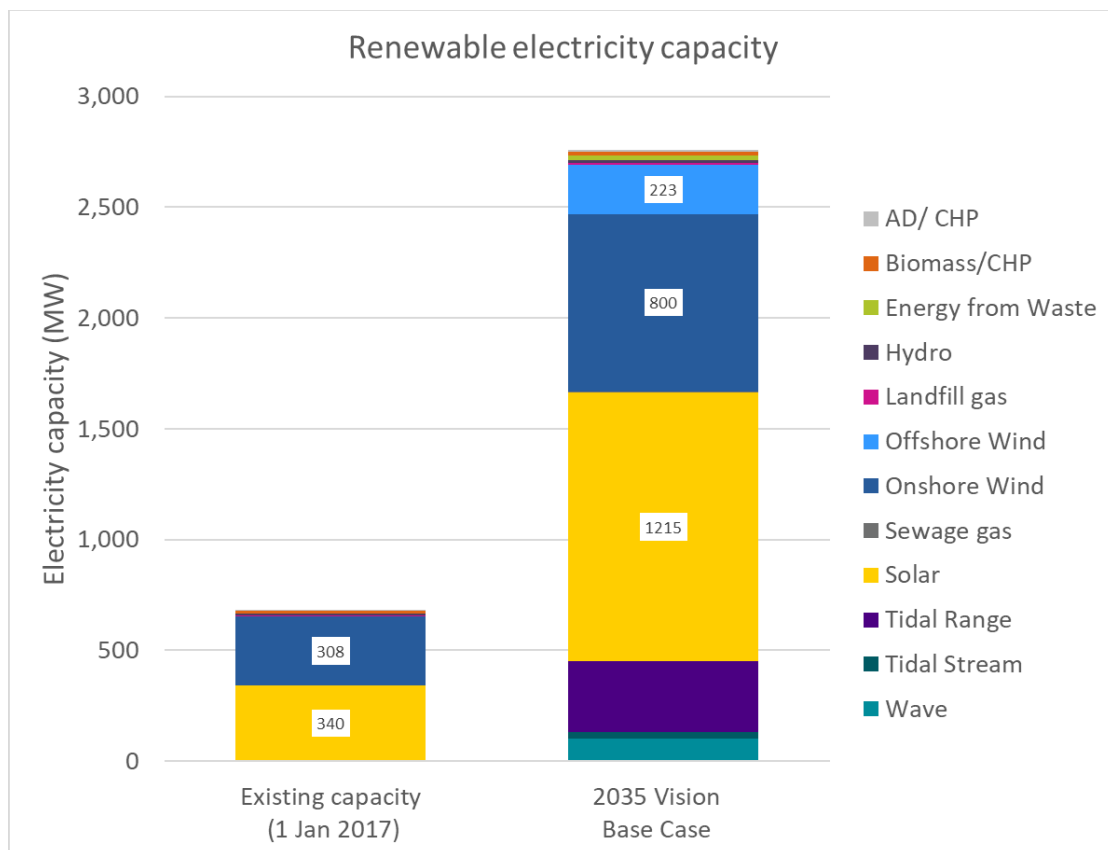
Figure 20: SBCR Energy Vision 2035 - Base Case renewable energy capacity mix
