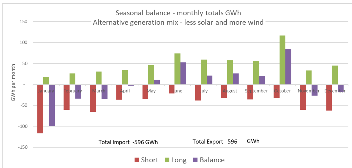
Figure 53: System balance with an alternative energy mix with more wind and less solar
