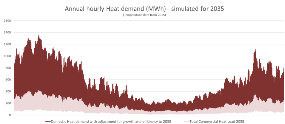
Figure 15: Simulated hourly heat demand for 2035 based on 2015 temperature and demand profiles
