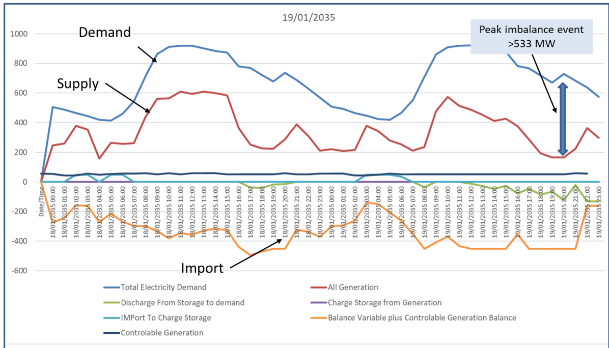
Figure 54 Simulated peak imbalance 19th January 2035
