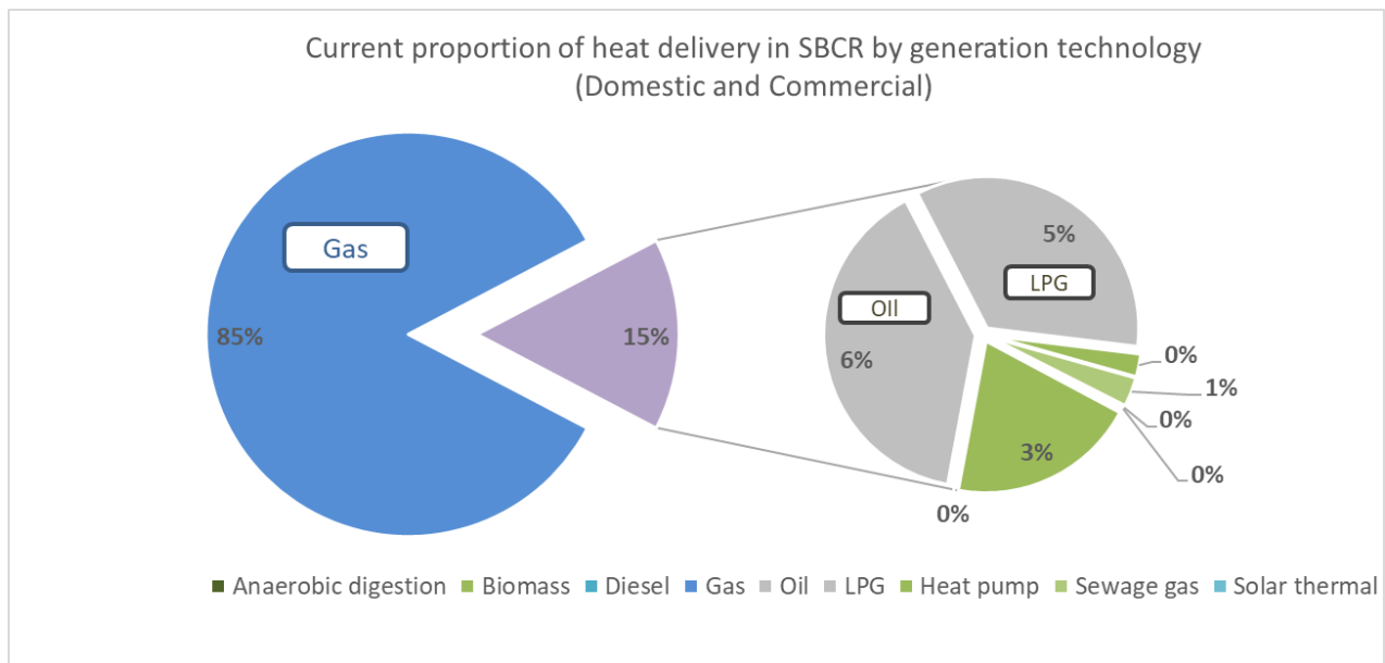
Figure 27: The current heat provision in the SBCR is dominated by gas with circa 85% of heat, while oil and LPG are still widely used in off-gas grid areas
