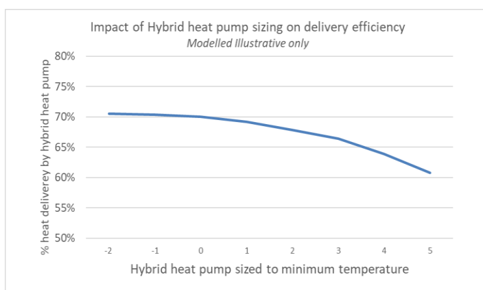
Figure 37: Impact of heat pump sizing on backup system usage
