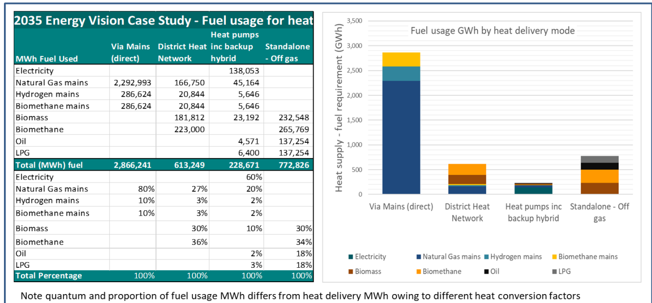
Figure 32: Energy system vision fuel usage in heat delivery
