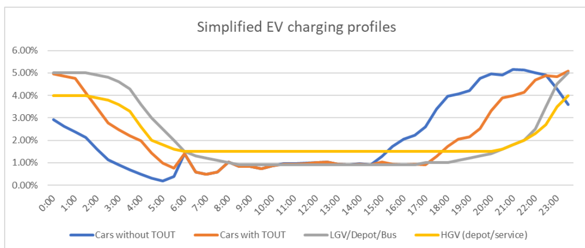
Figure 43: Vehicle charging profiles for demand modelling - before flexibility demand side response
