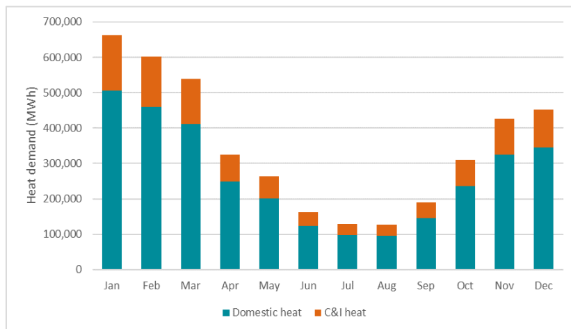
Figure 14: Monthly heat demand totals for SBCR in 2035 for domestic and C&I consumption (note in the fictional weather year used – based on 2015 temp. data - December was mild with a late spring).
