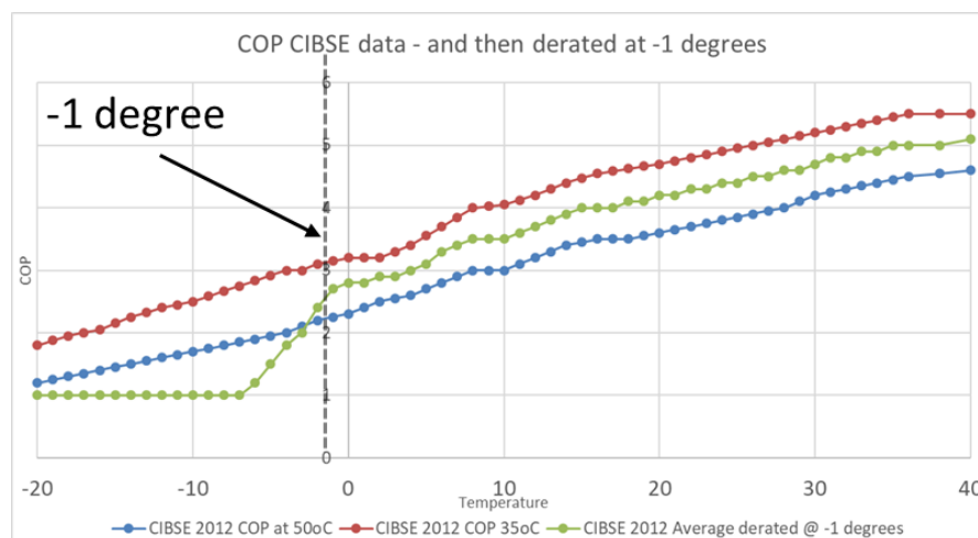
Figure 35: Relationship of COP to outside temperature and system sizing
