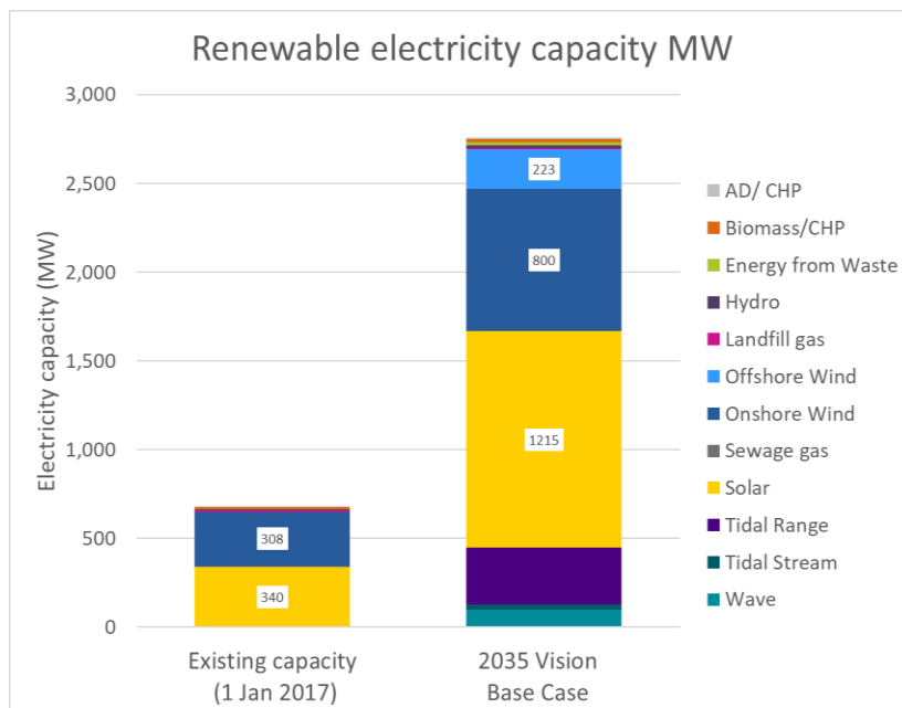
Figure 2: SBCR Energy Vision 2035 - Base case renewable electricity capacity mix
