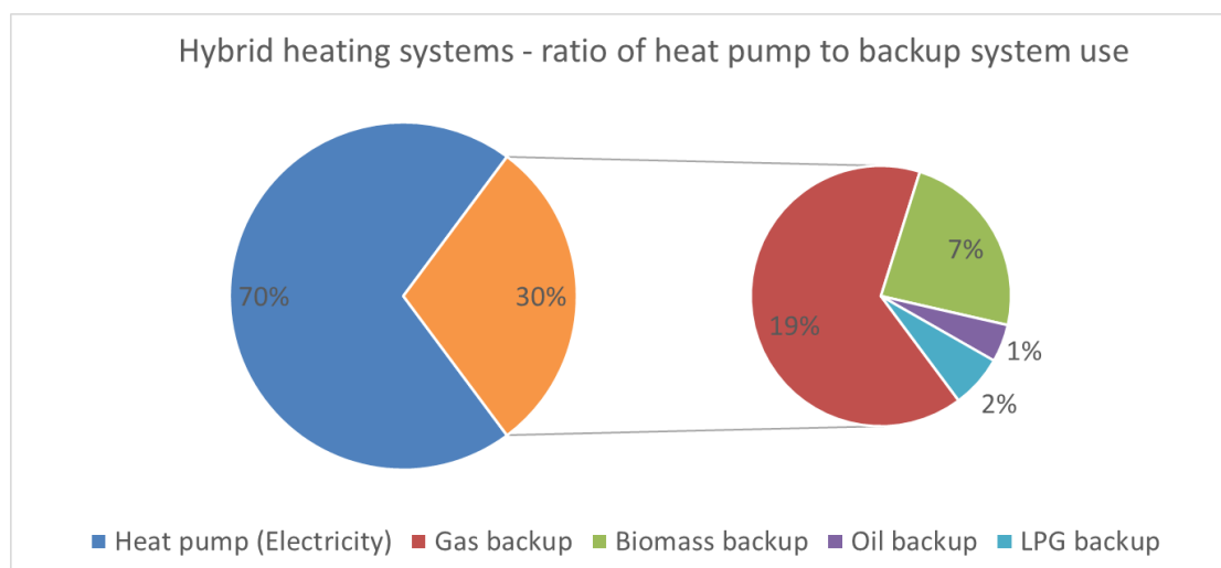
Figure 36: Modelled data showing ration of heat pump v backup system usage
